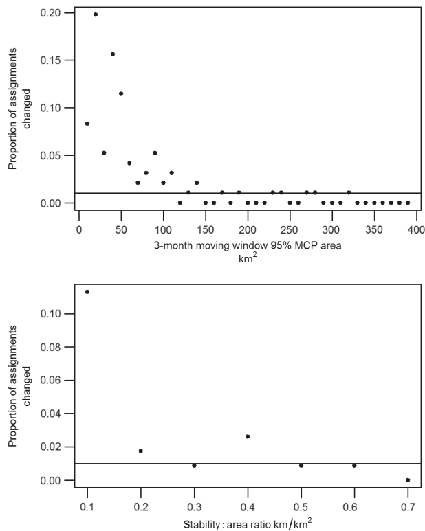
Figure 5. Sensitivity analysis plots for three-month moving window 95% MCP home range area (top) and the stability:area ratio ( \frac{d}{A} = \frac{\text{distance between successive monthly activity centers}}{95\% \text{ monthly MCP}} , bottom).
